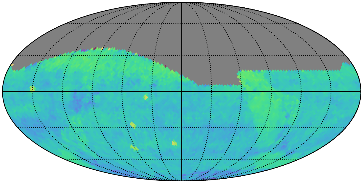
ddf_acor_sf15_lsf30_lsr20_v3.4_10yrs (g or r or i): PairFraction
