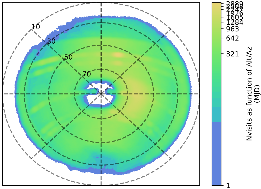
ddf_acor_sf15_ls30_lsr20_v3.4_10yrs z: Nvisits as function of Alt/Az
