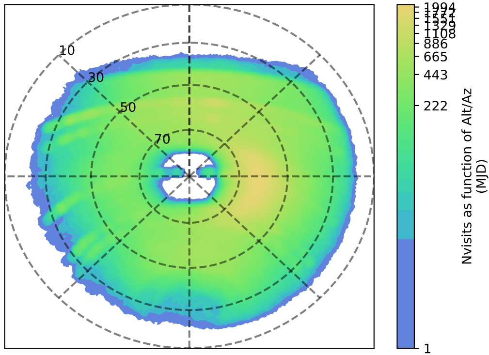
ddf_acor_sf15_lsf30_lsr20_v3.4_10yrs y: Nvisits as function of Alt/Az
