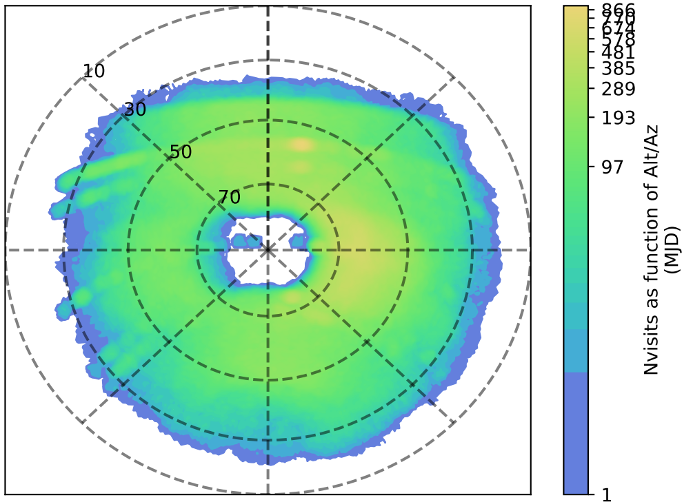
ddf_acor_sf15_lsf30_lsr20_v3.4_10yrs u: Nvisits as function of Alt/Az
