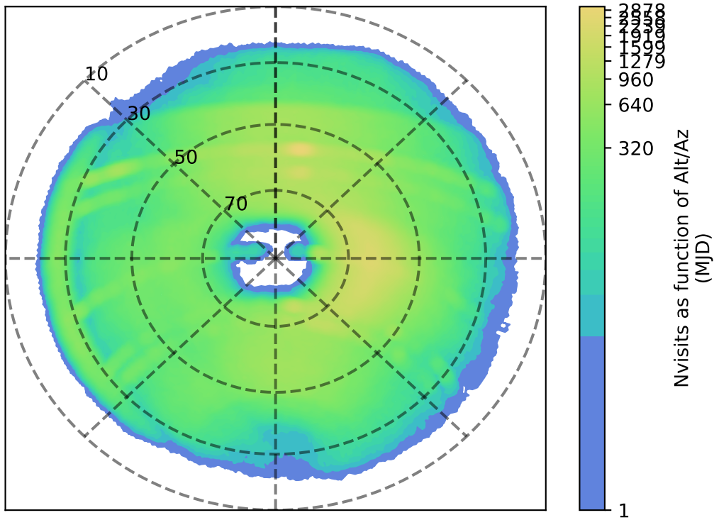
ddf_acor_sf15_ls30_lsr20_v3.4_10yrs r: Nvisits as function of Alt/Az
