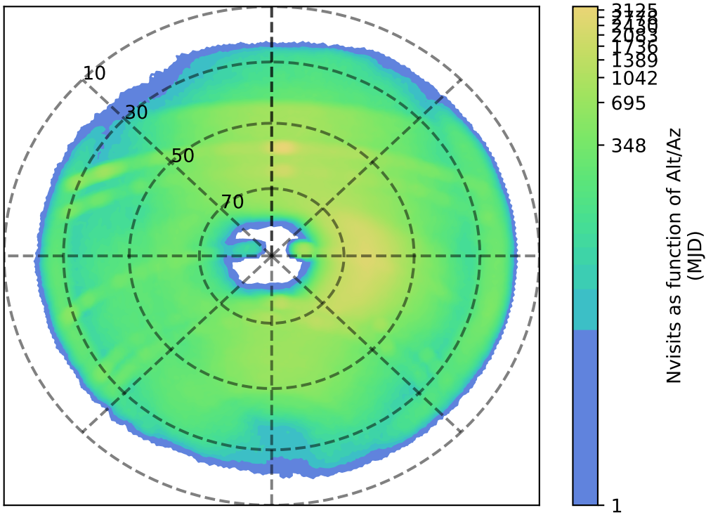
ddf_acor_sf15_ls30_lsr20_v3.4_10yrs i: Nvisits as function of Alt/Az
