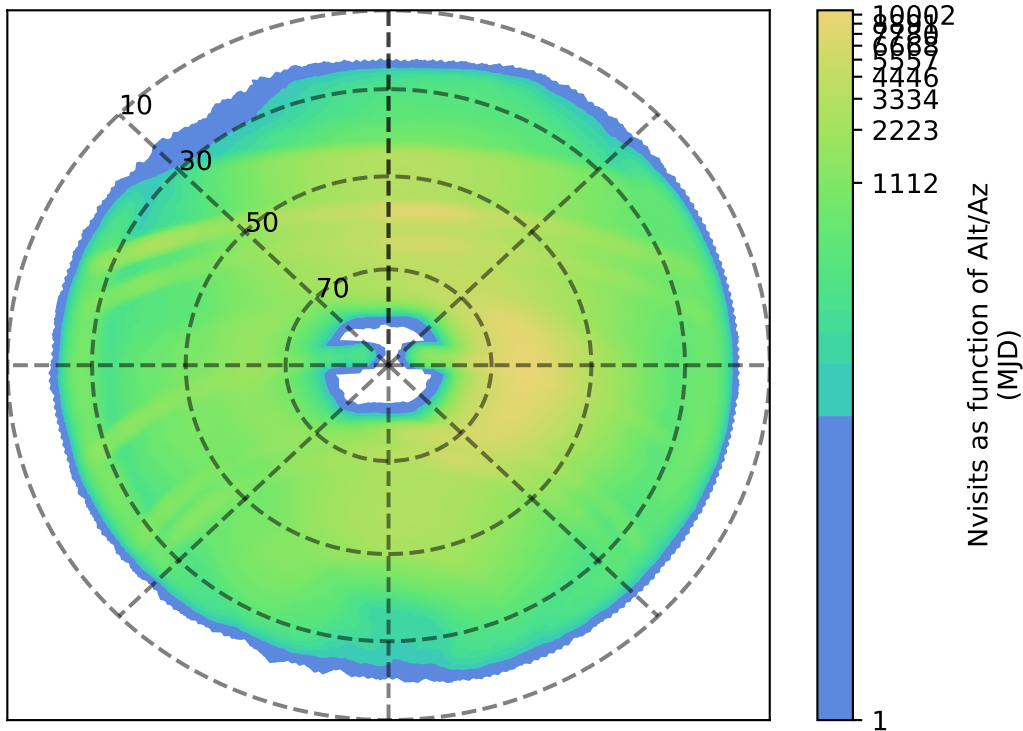
ddf_acor_sf15_lsf30_lsr20_v3.4_10yrs : Nvisits as function of Alt/Az
