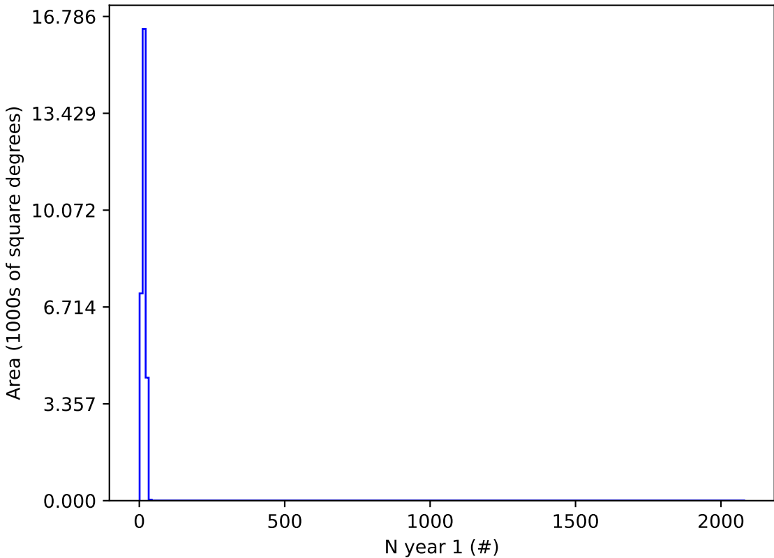
ddf_acor_sf15_lsf30_lsr20_v3.4_10yrs r and night < 365: N year 1
