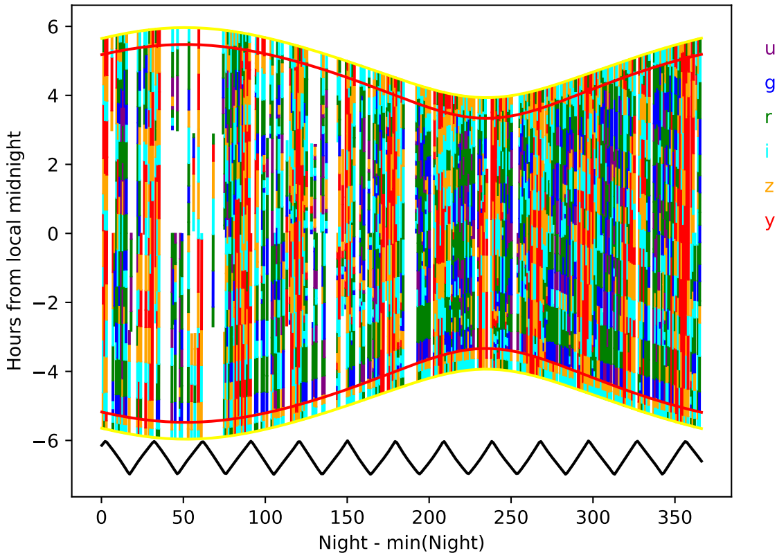
ddf_acor_sf15_lsf30_lsr20_v3.4_10yrs year 9-10: Hourglass
