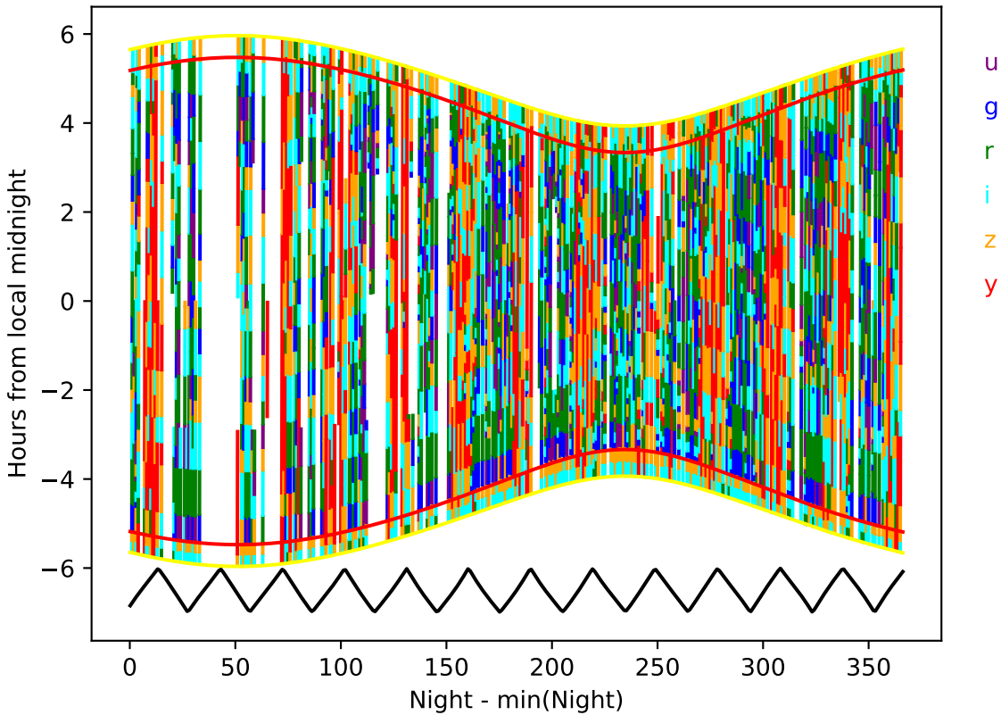
ddf_acor_sf15_lsf30_lsr20_v3.4_10yrs year 8-9: Hourglass
