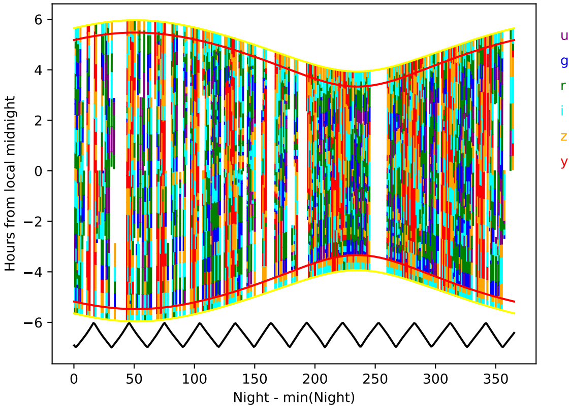
ddf_acor_sf15_lsf30_lsr20_v3.4_10yrs year 5-6: Hourglass
