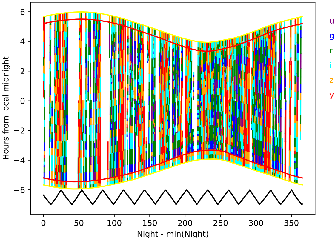
ddf_acor_sf15_lsf30_lsr20_v3.4_10yrs year 4-5: Hourglass
