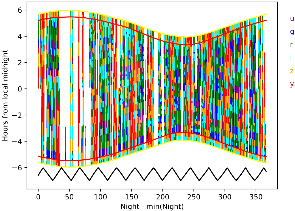
ddf_acor_sf15_lsf30_lsr20_v3.4_10yrs year 3-4: Hourglass
