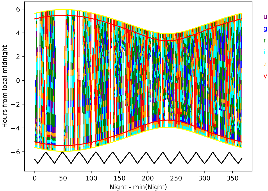
ddf_acor_sf15_lsf30_lsr20_v3.4_10yrs year 2-3: Hourglass
