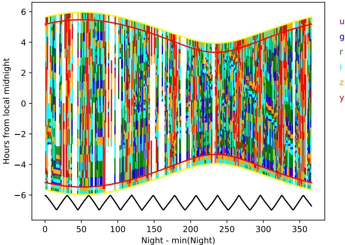
ddf_acor_sf15_lsf30_lsr20_v3.4_10yrs year 1-2: Hourglass
