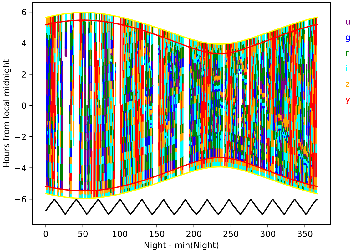
ddf_acor_sf15_lsf30_lsr20_v3.4_10yrs year 0-1: Hourglass
