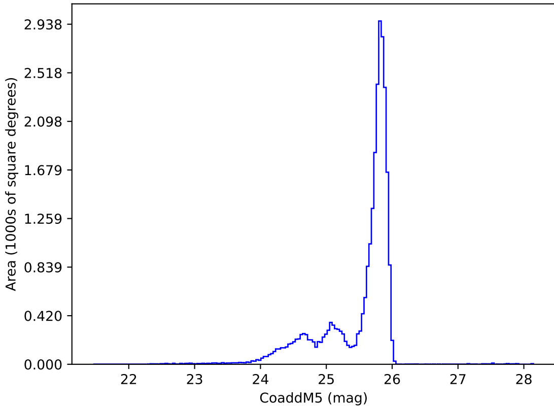
ddf_acor_sf15_lsf30_lsr20_v3.4_10yrs z: CoaddM5
