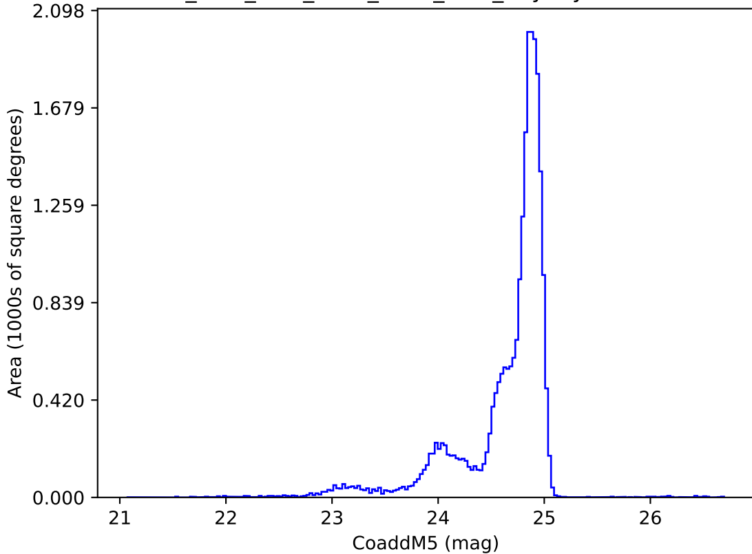
ddf_acor_sf15_lsf30_lsr20_v3.4_10yrs y: CoaddM5
