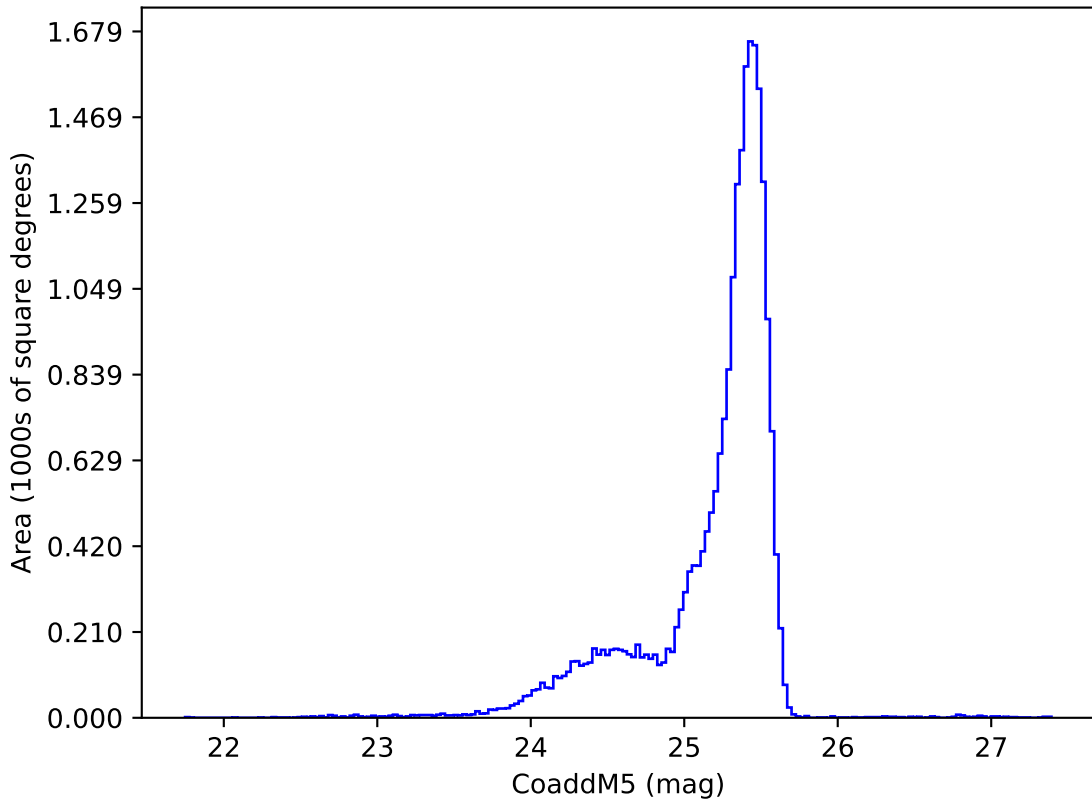
ddf_acor_sf15_lsf30_lsr20_v3.4_10yrs u: CoaddM5
