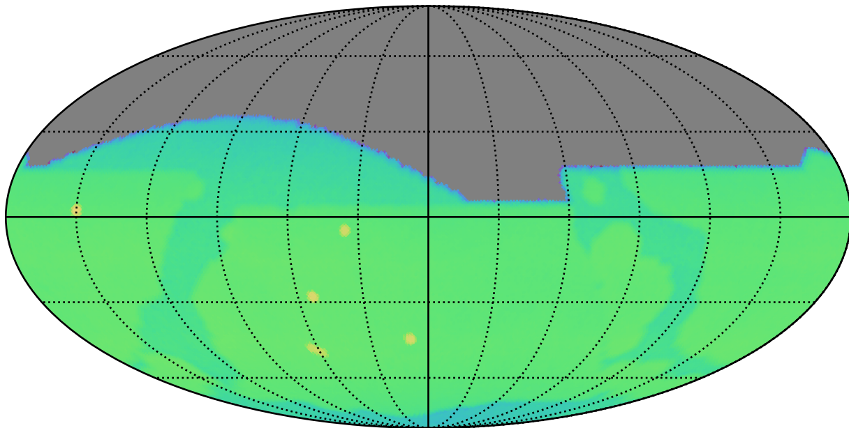
ddf_acor_sf15_lsf30_lsr20_v3.4_10yrs : CoaddM5
