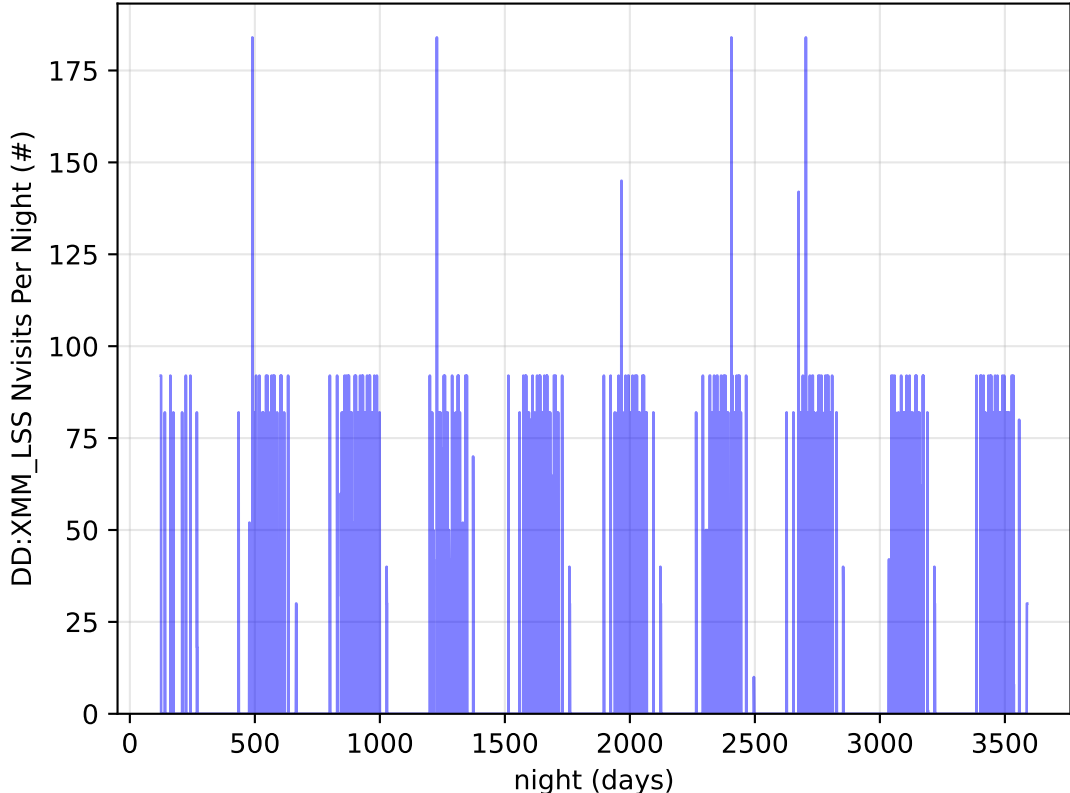
ddf_acor_sf15_lsf30_lsr20_v3.4_10yrs all bands: DD:XMM_LSS Nvisits Per Night
