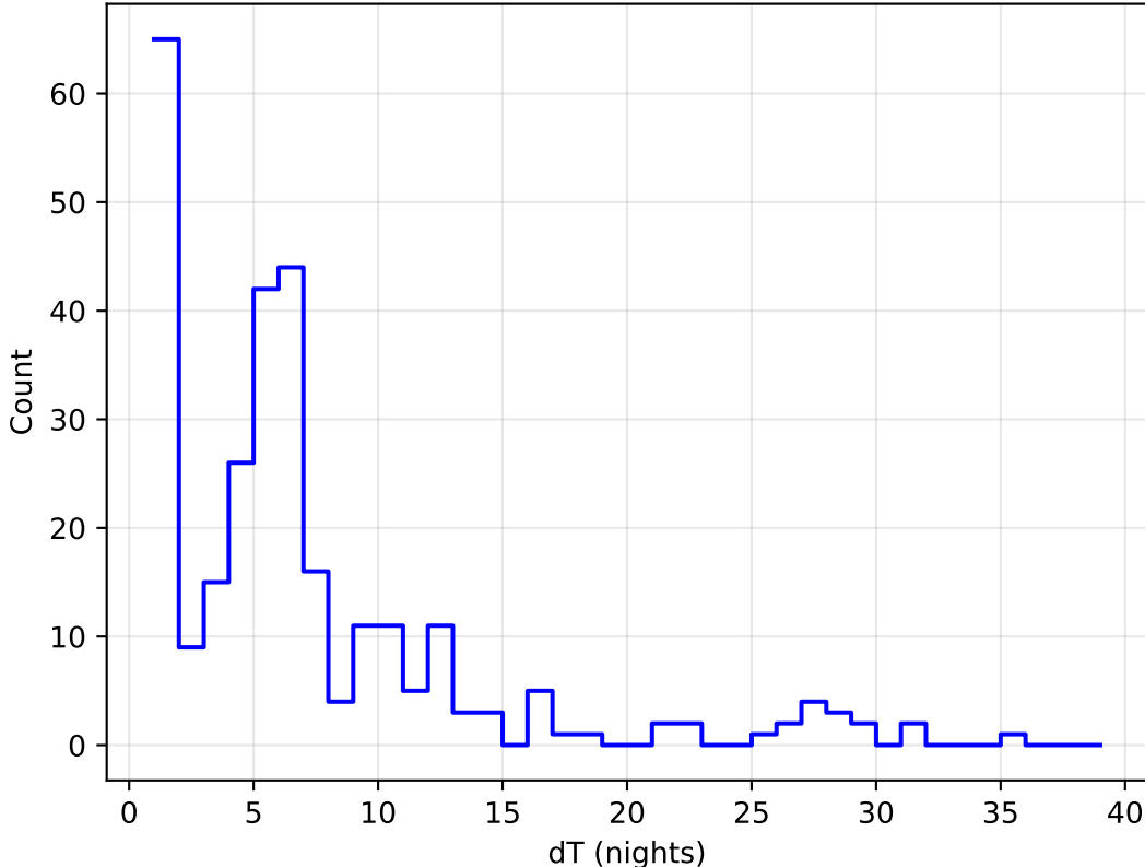
ddf_acor_sf15_lsf30_lsr20_v3.4_10yrs all bands: DD:XMM_LSS Delta Nights Histogram
