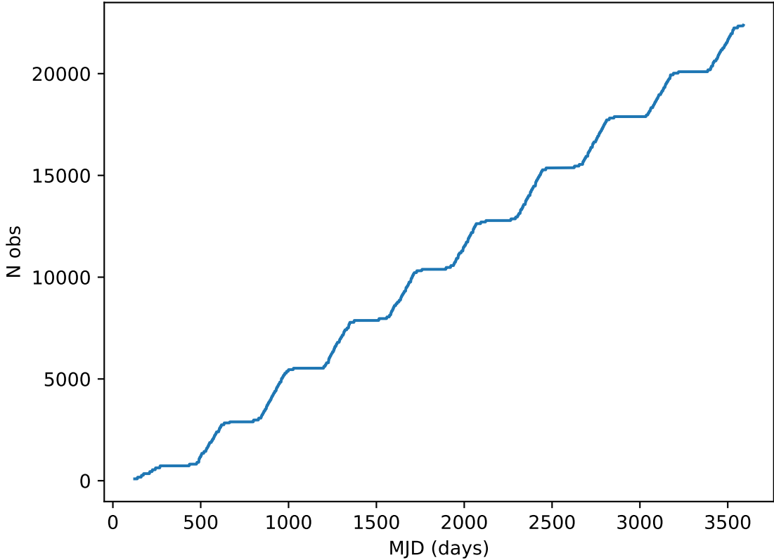
ddf_acor_sf15_lsf30_lsr20_v3.4_10yrs all bands: DD:XMM_LSS Cumulative NVisits
