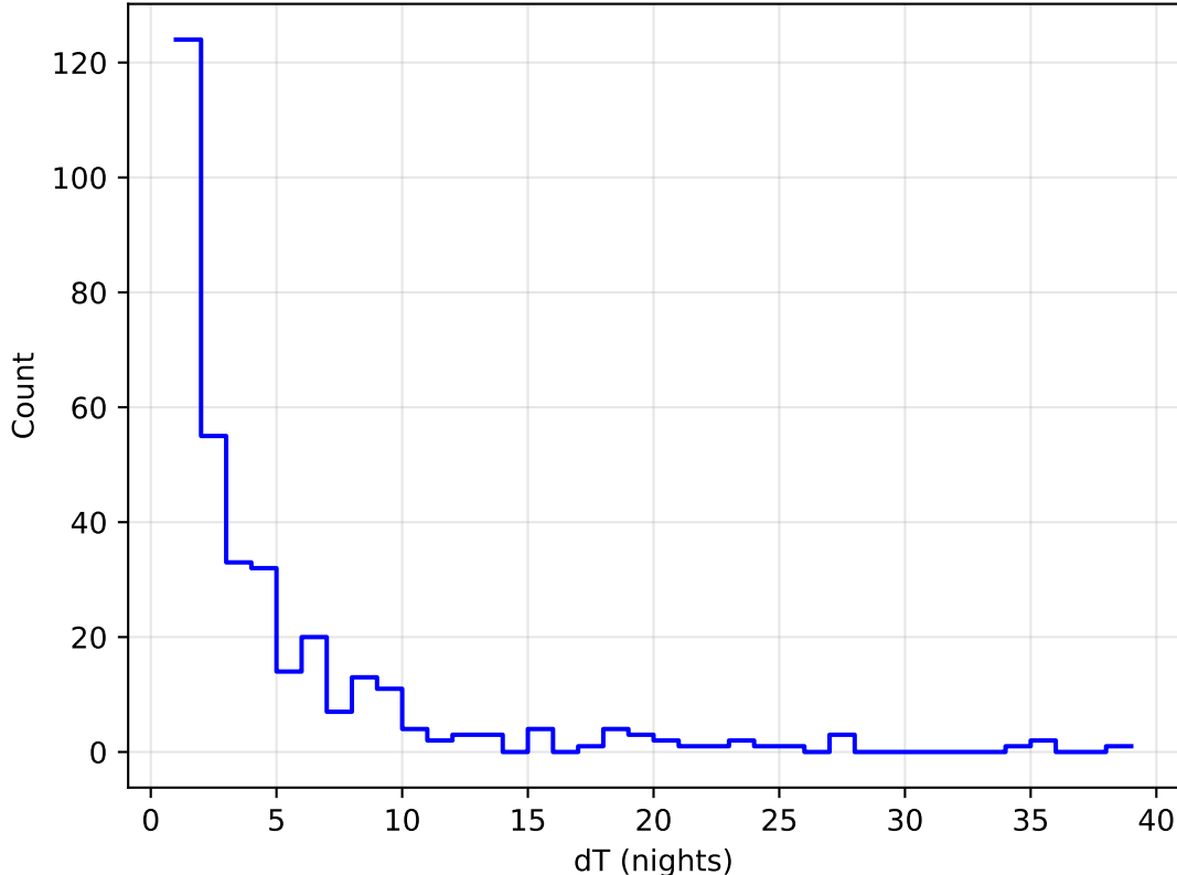
ddf_acor_sf15_lsf30_lsr20_v3.4_10yrs all bands: DD:WFD Delta Nights Histogram
