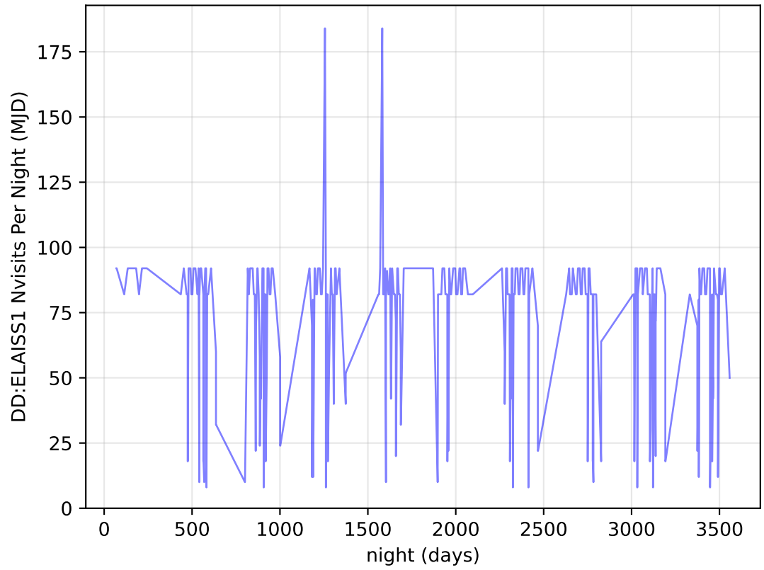
ddf_acor_sf15_lsf30_lsr20_v3.4_10yrs all bands: DD:ELAISS1 Nvisits Per Night
