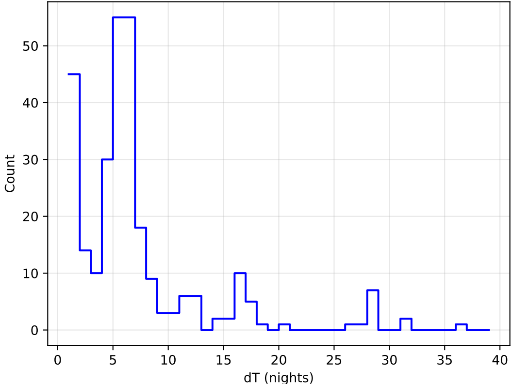
ddf_acor_sf15_lsf30_lsr20_v3.4_10yrs all bands: DD:ELAISS1 Delta Nights Histogram
