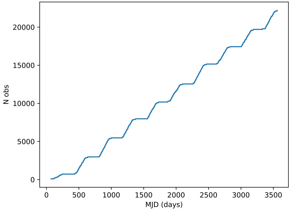
ddf_acor_sf15_lsf30_lsr20_v3.4_10yrs all bands: DD:ELAISS1 Cumulative NVisits
