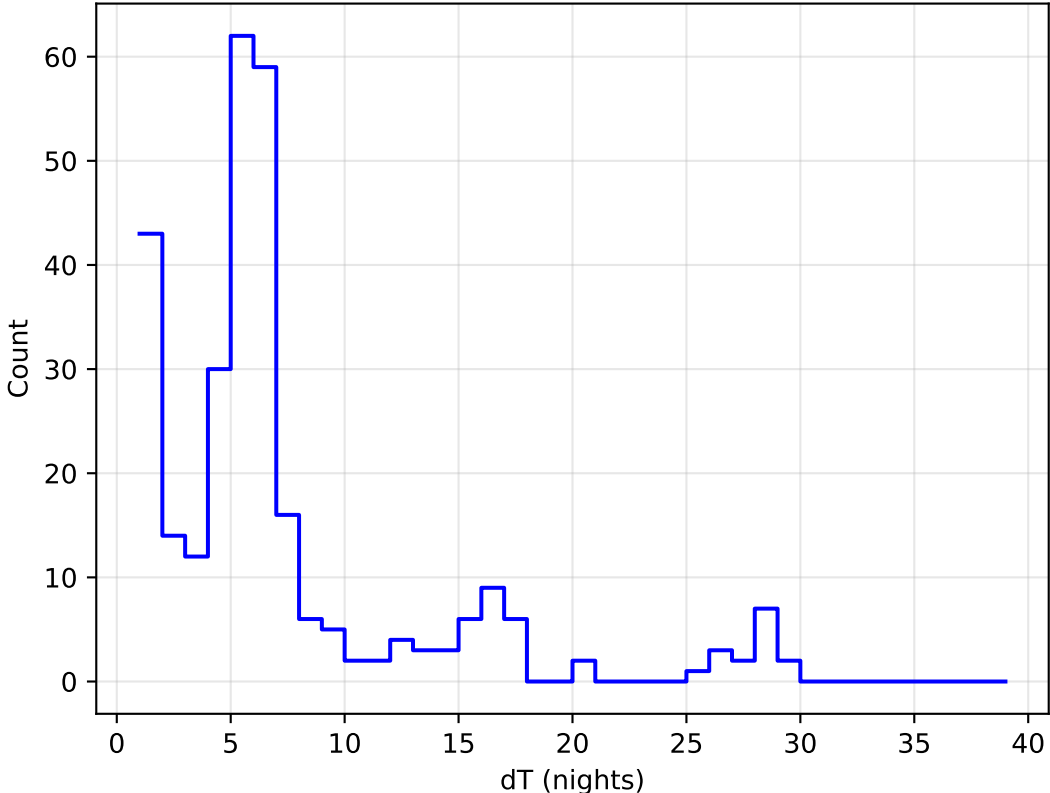
ddf_acor_sf15_lsf30_lsr20_v3.4_10yrs all bands: DD:EDFS Delta Nights Histogram
