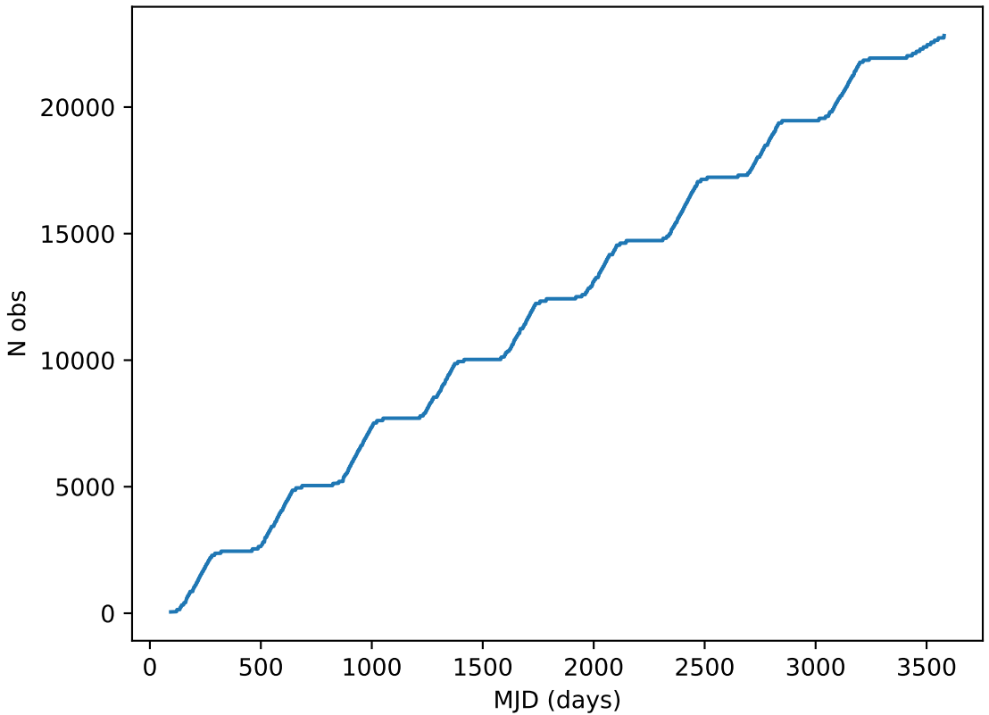
ddf_acor_sf15_lsf30_lsr20_v3.4_10yrs all bands: DD:EDFS Cumulative NVisits
