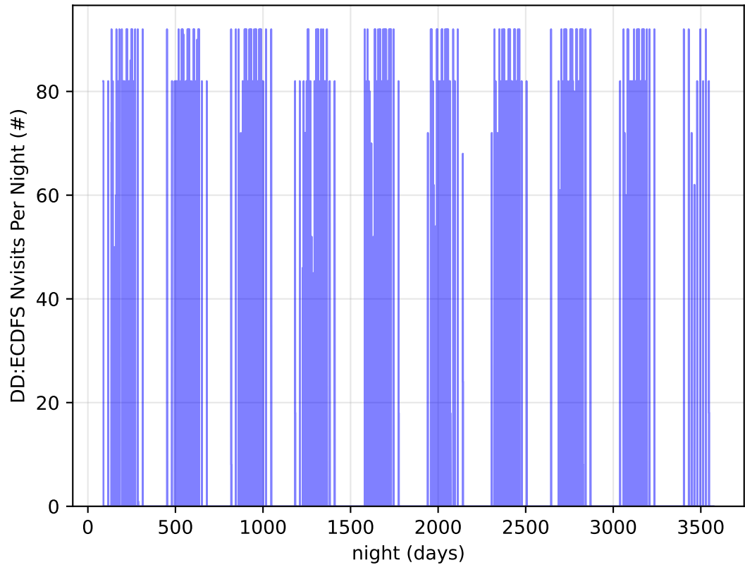
ddf_acor_sf15_lsf30_lsr20_v3.4_10yrs all bands: DD:ECDFS Nvisits Per Night
