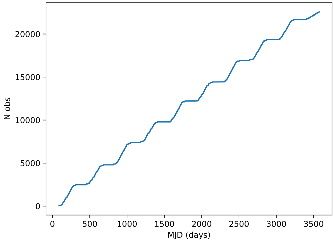
ddf_acor_sf15_lsf30_lsr20_v3.4_10yrs all bands: DD:ECDFS Cumulative NVisits
