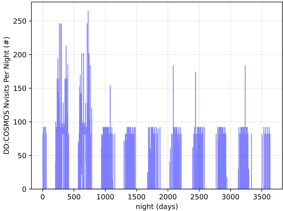
ddf_acor_sf15_lsf30_lsr20_v3.4_10yrs all bands: DD: COSMOS Nvisits Per Night
