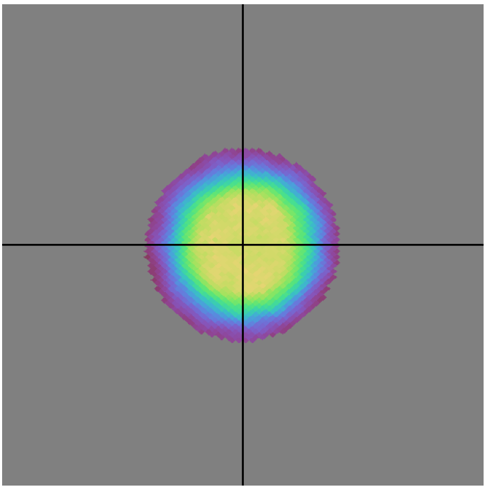
ddf_acor_sf15_lsf30_lsr20_v3.4_10yrs all bands: DD:COSMOS N Unique Nights
