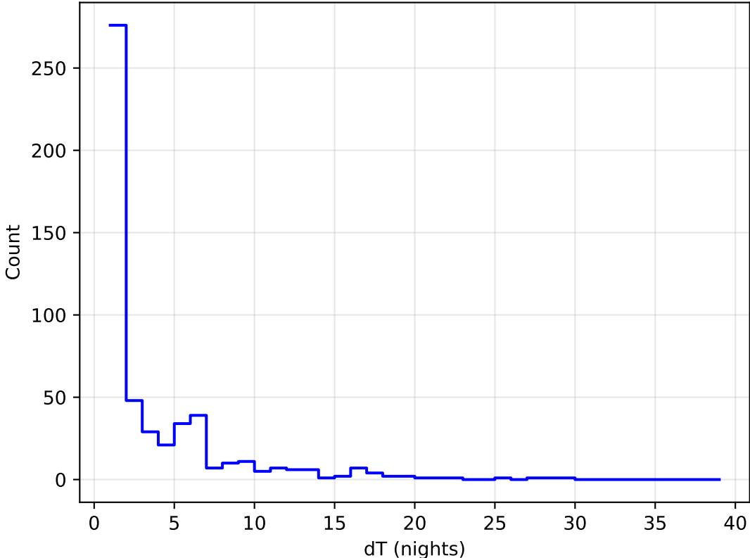
ddf_acor_sf15_Isf30_Isr20_v3.4_10yrs all bands: DD: COSMOS Delta Nights Histogram
