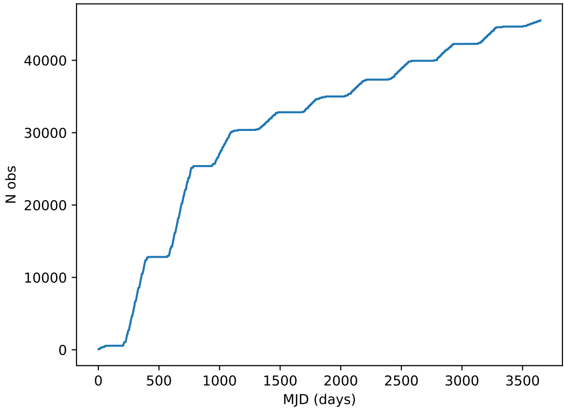
ddf_acor_sf15_lsf30_lsr20_v3.4_10yrs all bands: DD: COSMOS Cumulative NVisits
