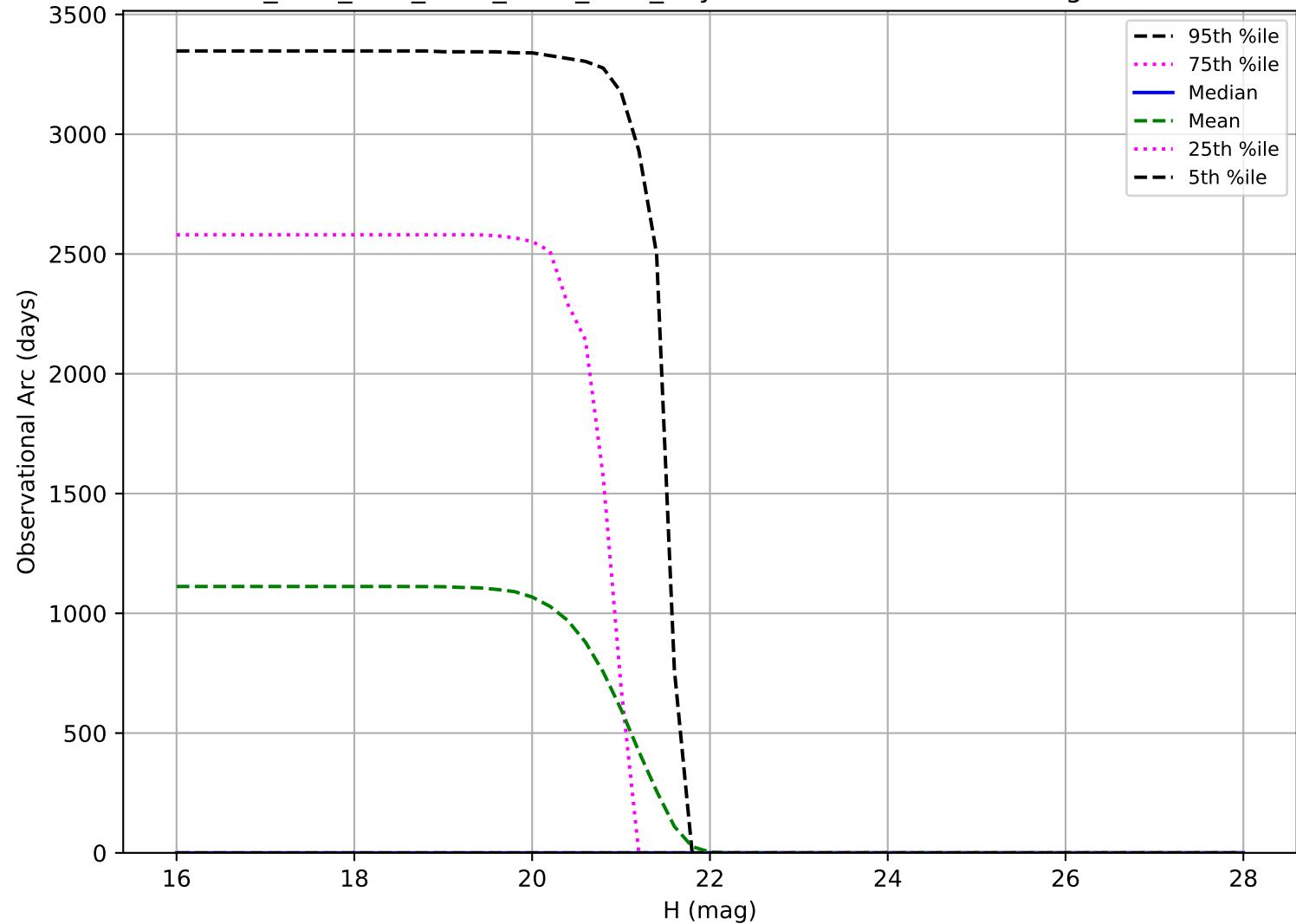
ddf_acor_sf15_lsf30_lsr10_v3.4_10yrs: Observational Arc Length Vatira
