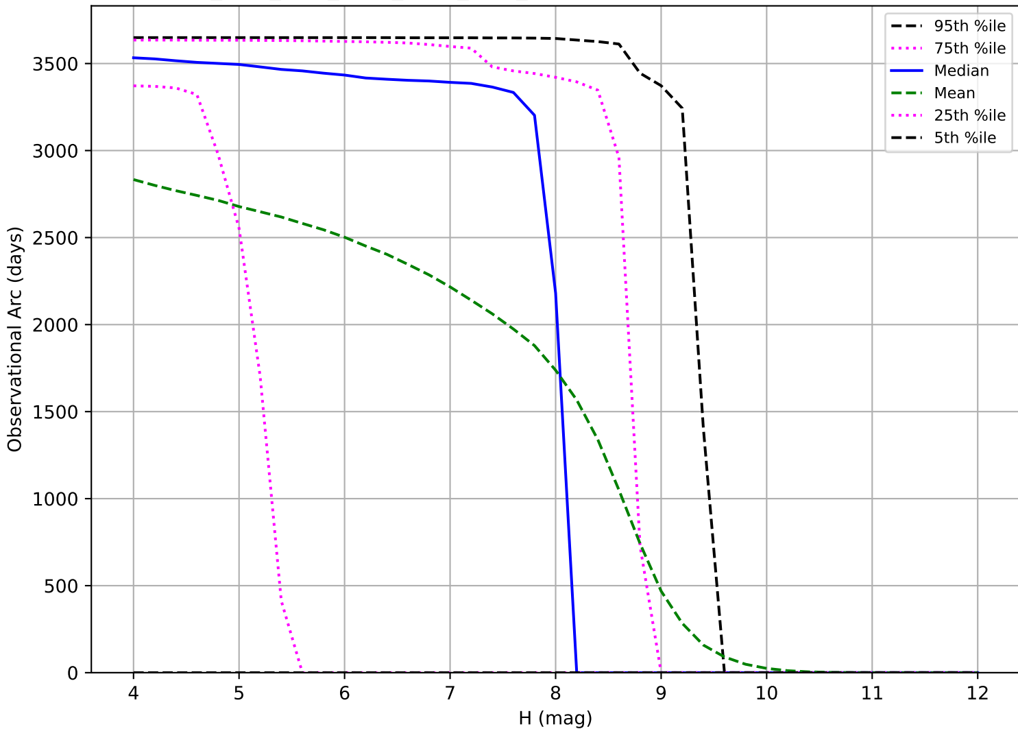
ddf_acor_sf15_lsf30_lsr10_v3.4_10yrs: Observational Arc Length TNO
