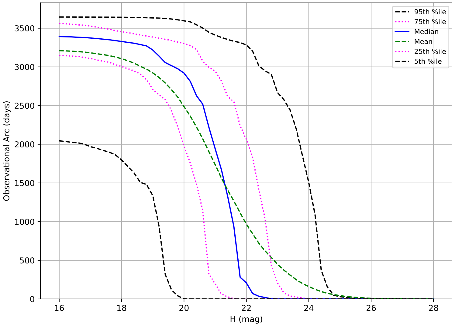
ddf_acor_sf15_lsf30_lsr10_v3.4_10yrs: Observational Arc Length PHA
