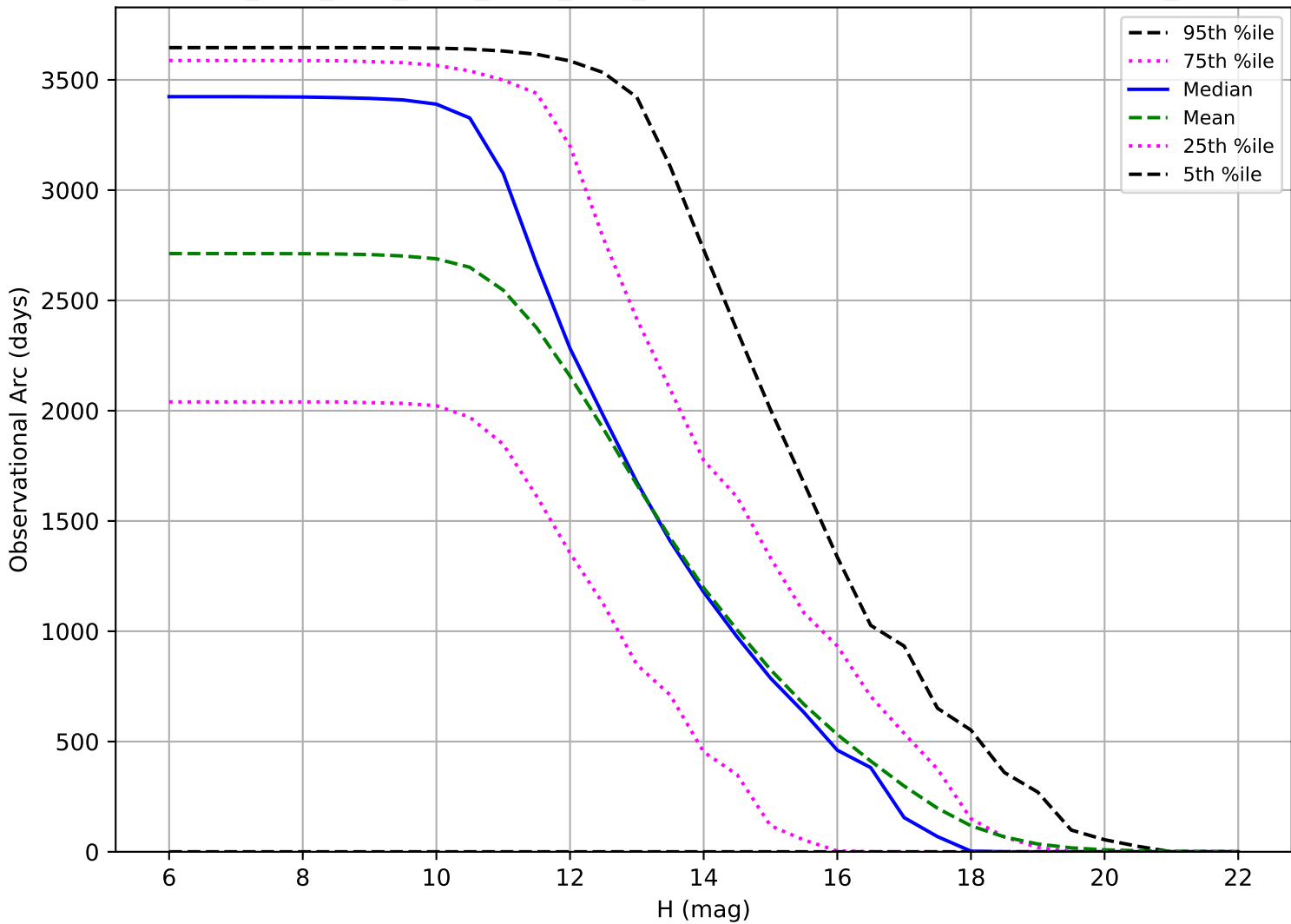
ddf_acor_sf15_lsf30_lsr10_v3.4_10yrs: Observational Arc Length OCC_r5
