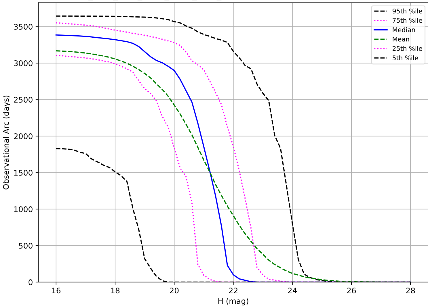
ddf_acor_sf15_lsf30_lsr10_v3.4_10yrs: Observational Arc Length NEO
