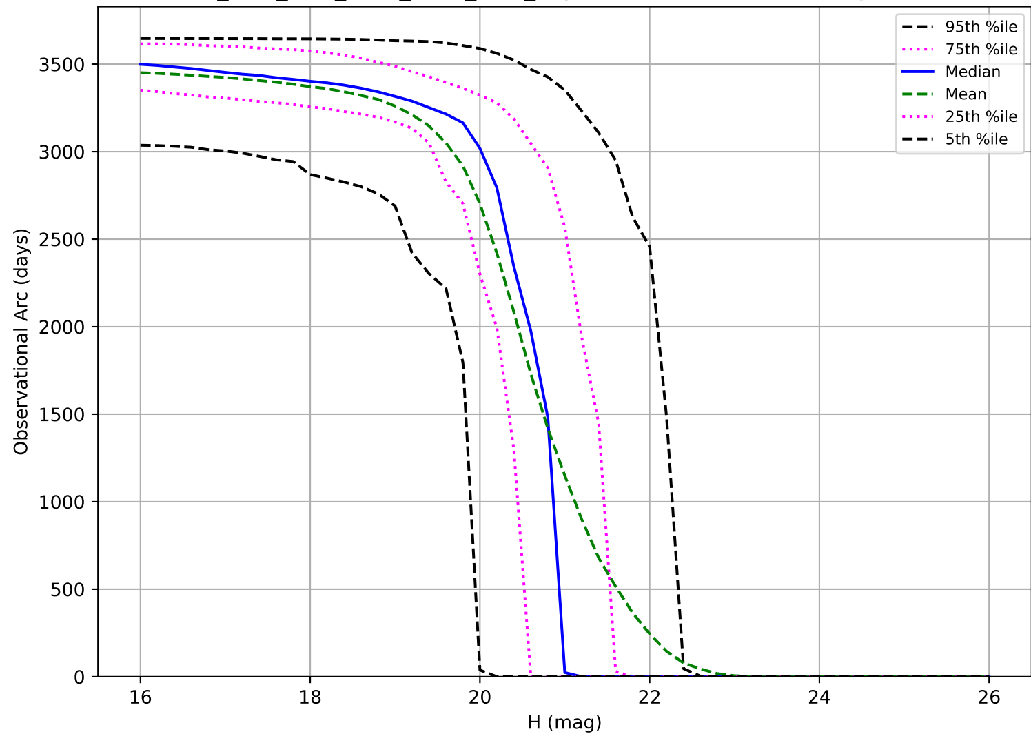
ddf_acor_sf15_lsf30_lsr10_v3.4_10yrs: Observational Arc Length MBA
