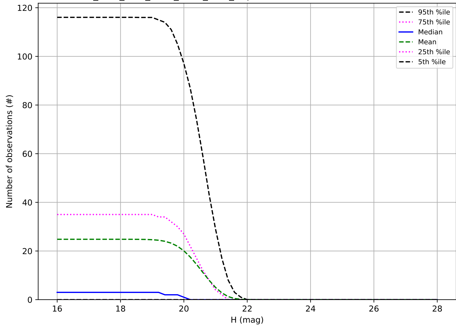
ddf_acor_sf15_lsf30_lsr10_v3.4_10yrs: Number of observations Vatira
