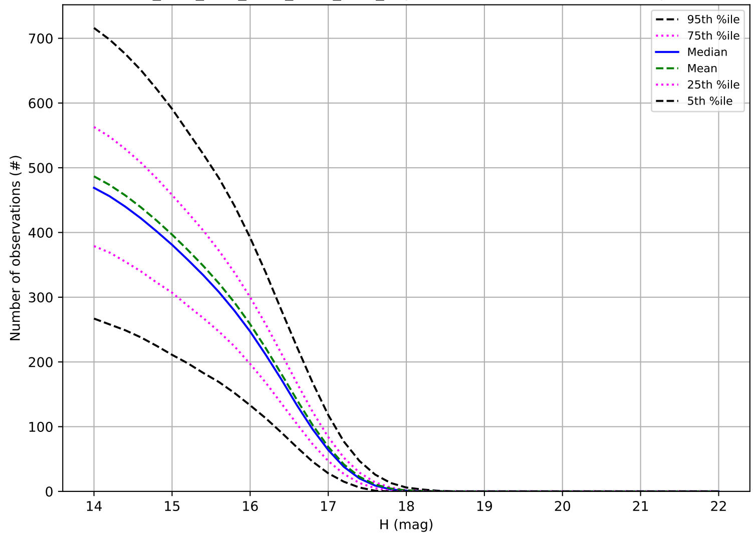
ddf_acor_sf15_lsf30_lsr10_v3.4_10yrs: Number of observations Trojan
