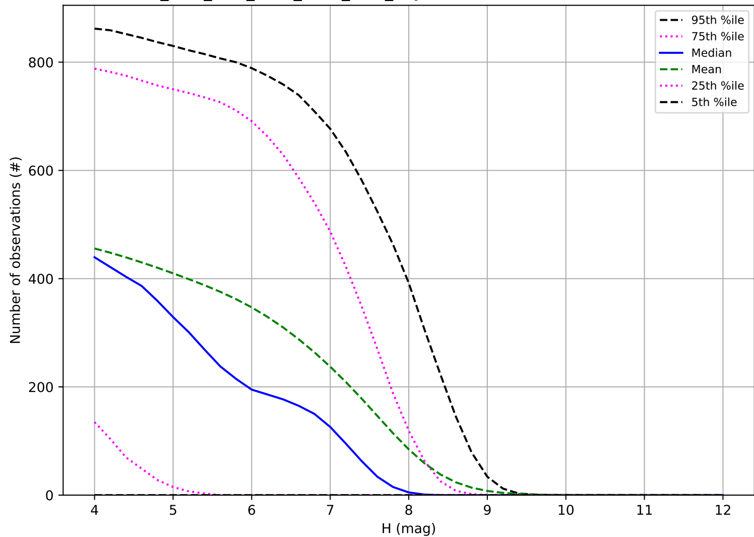
ddf_acor_sf15_lsf30_lsr10_v3.4_10yrs: Number of observations TNO
