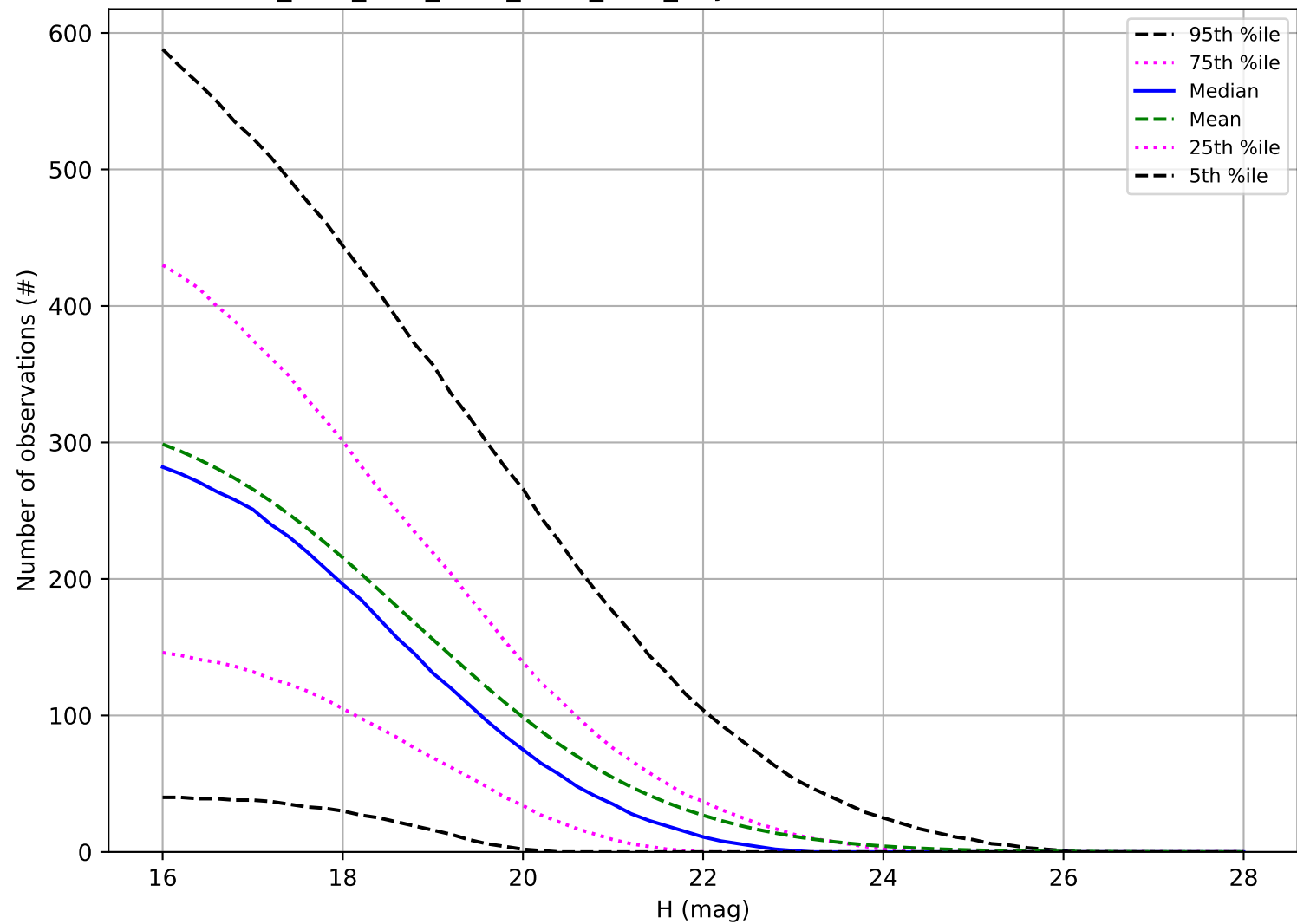
ddf_acor_sf15_lsf30_lsr10_v3.4_10yrs: Number of observations PHA
