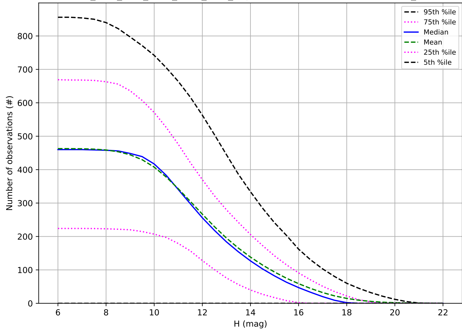
ddf_acor_sf15_lsf30_lsr10_v3.4_10yrs: Number of observations OCC_r5
