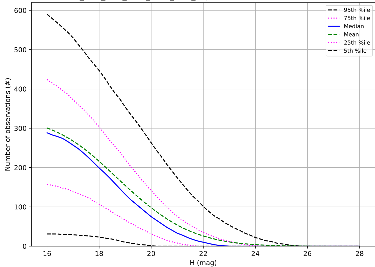
ddf_acor_sf15_lsf30_lsr10_v3.4_10yrs: Number of observations NEO
