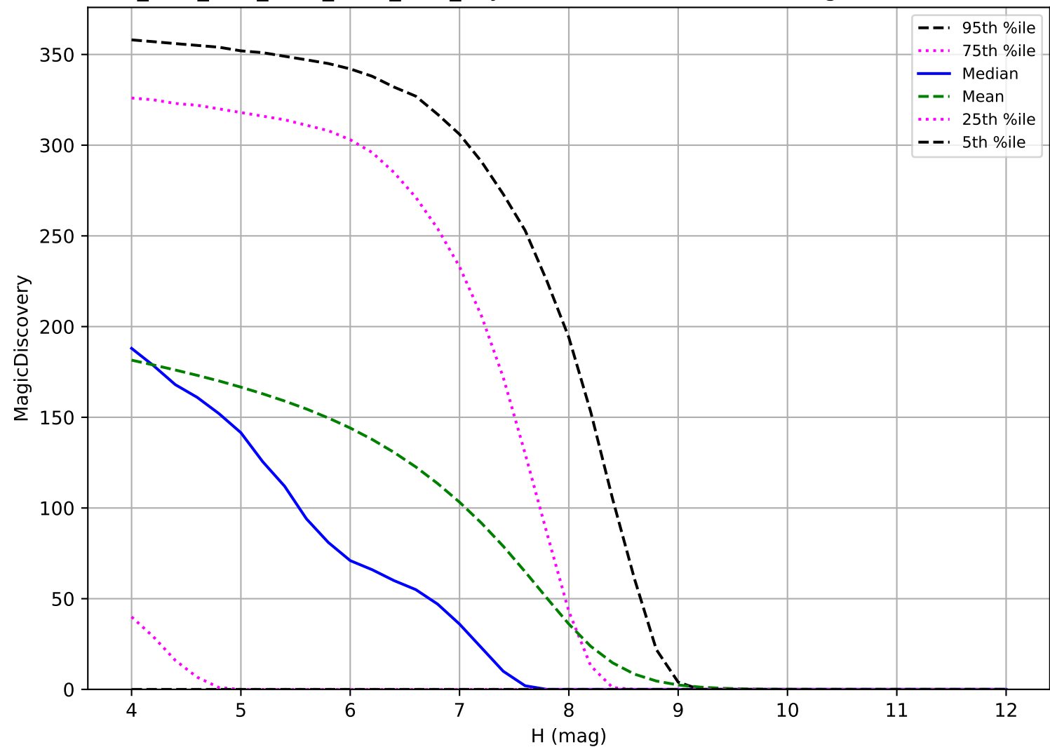
ddf_acor_sf15_lsf30_lsr10_v3.4_10yrs: TNO 6 detections in 60 nights detection loss
