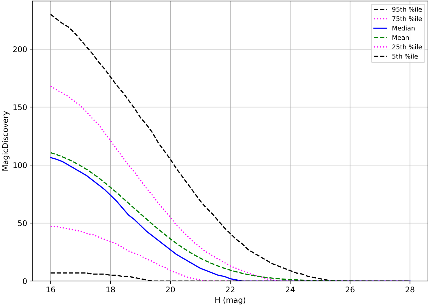
ddf_acor_sf15_lsf30_lsr10_v3.4_10yrs: PHA 6 detections in 60 nights detection loss
