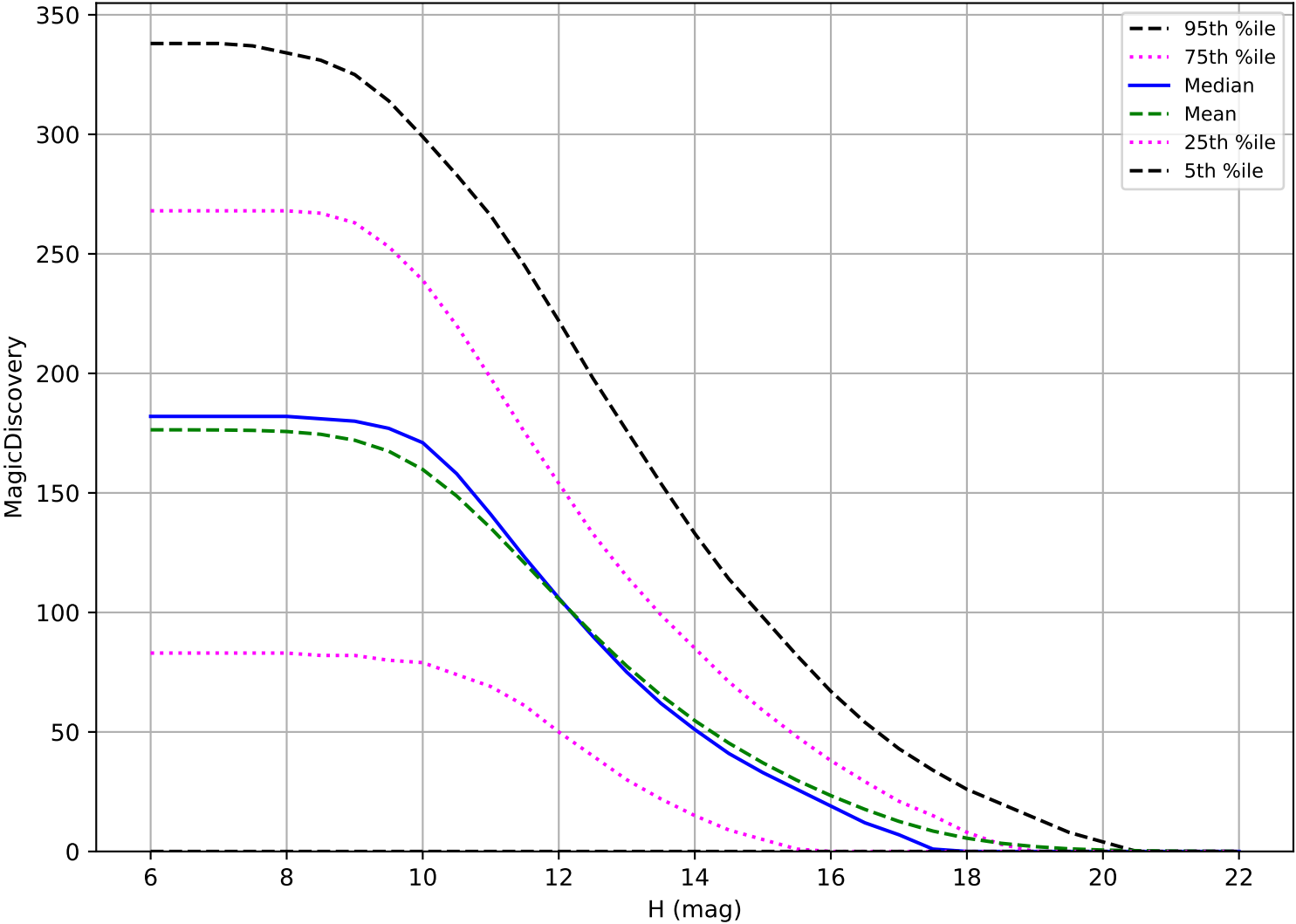
ddf_acor_sf15_lsf30_lsr10_v3.4_10yrs: OCC_r5 6 detections in 60 nights detection loss
